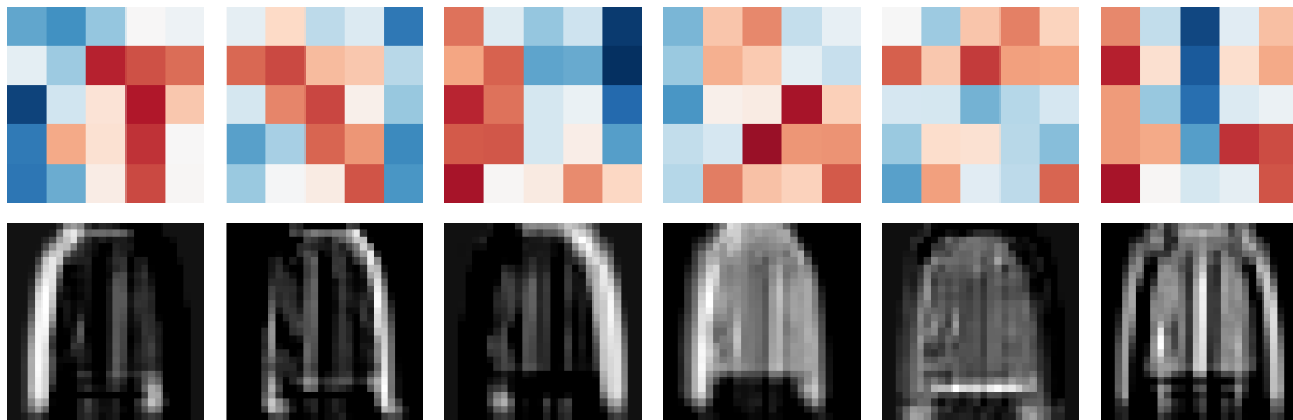
Figure 8.5.: What LeNet learned to look for. Top: six first-layer 5 \times 5 kernels (red positive, blue negative). Bottom: their feature maps on the same validation coat used in Figure 8.3, whose sleeves and torso make spatial responses easier to compare than the earlier sandal. The maps respond differently, but several kernels remain diffuse and should not be over-interpreted.
