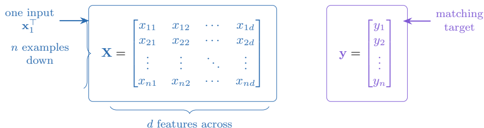
Figure 1.1.: Stacking examples turns a dataset into two aligned objects: one row of \mathbf{X} per input and one entry of \mathbf{y} per desired output. Colour will keep these roles visible in the equations that follow.
