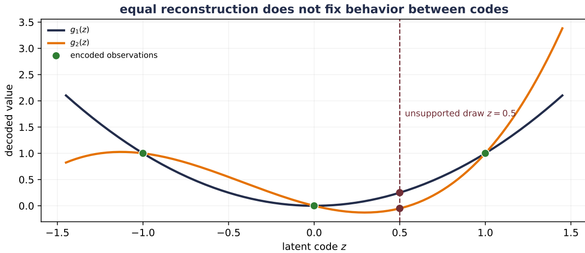
Figure 9.9.: Reconstruction does not identify a latent sampler or a unique decoder away from observed codes. The two displayed decoders agree exactly at z equal to -1, 0, and 1, so both have zero reconstruction error on the three targets. They disagree between and beyond those codes; at z = 0.5 their outputs are 0.25 and -0.05.
