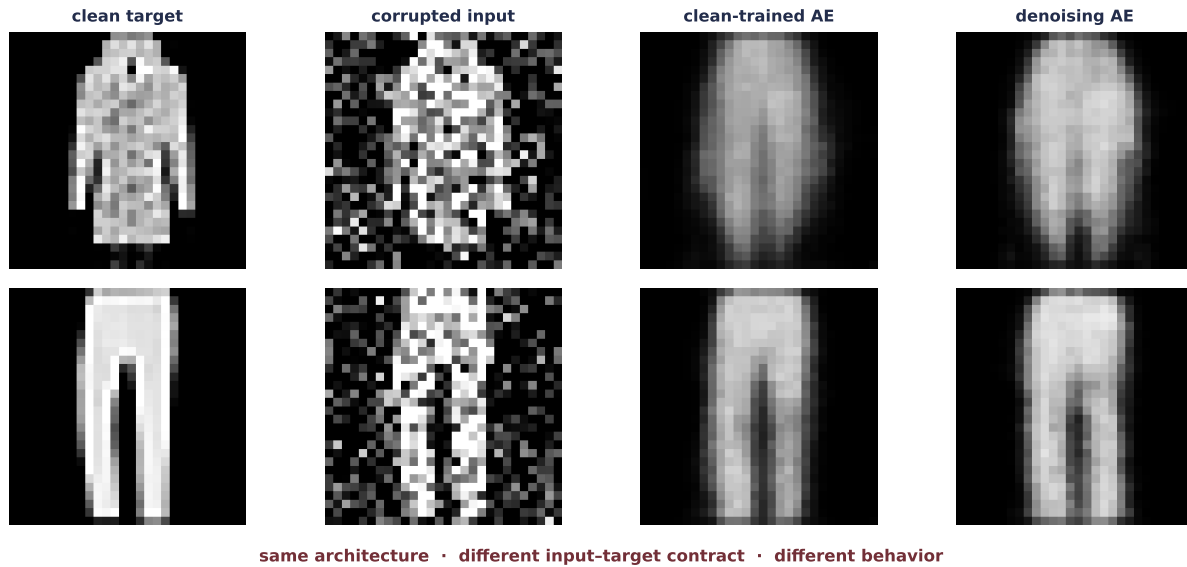
Figure 9.10.: The input–target contract determines what the same convolutional autoencoder learns to preserve. Before reconstruction, Gaussian corruption has test MSE 0.068601. Across seeds 6050–6054, the clean-trained autoencoder has mean clean/noisy-input test MSE 0.020701/0.033263 (SD 0.000565/0.003642). The denoising autoencoder has 0.026294/0.023810 (SD 0.001445/0.000775): it gives up some clean reconstruction accuracy to become better at the corruption it was trained to remove. This CPU Fashion-MNIST-subset study isolates a change in the training contract; it is not a universal ranking of denoisers.
