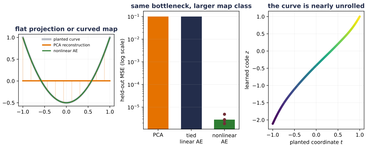
Figure 9.8.: A one-dimensional bottleneck behaves differently when its maps may bend. On the alternating held-out grid, rank-one PCA and the tied linear autoencoder both have MSE 0.100000 and their projectors agree to displayed precision. Across seeds 6050–6054, the nonlinear autoencoder has mean held-out MSE 0.000002815 (SD 0.000001223); the absolute Pearson correlation between its code and the planted coordinate has mean 0.992802 (SD 0.005513). This controlled curve and capacity-mismatched model show a mechanism, not a universal nonlinear-autoencoder advantage.
