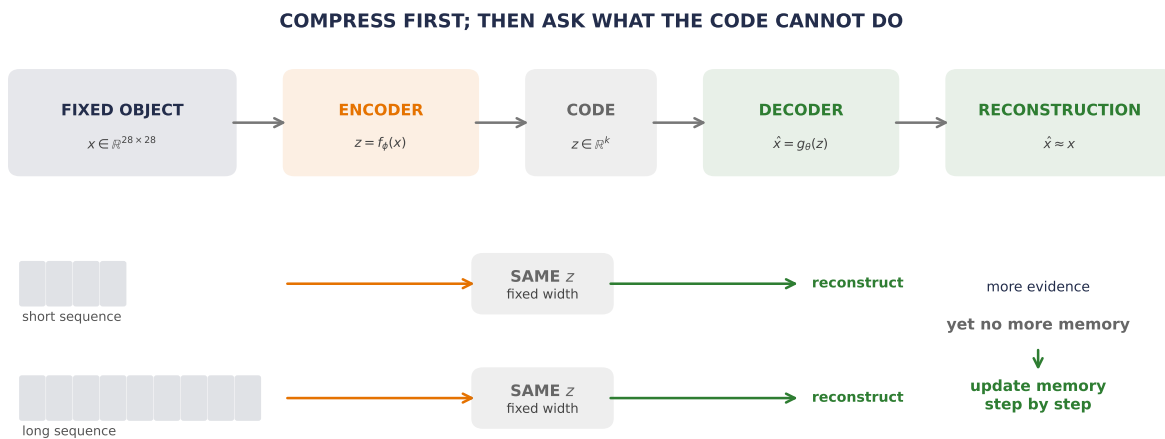
Figure 9.7.: The encoder–decoder detour solves one problem and reveals the next. A fixed-size object can be compressed into a code and reconstructed. Variable-length sequences can also be forced through one code, but the code’s width does not grow when the evidence does. The unmet need is a memory that can update as each new piece arrives.
