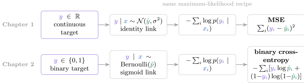
Figure 1.7.: The target type changes the conditional distribution and link function, but the maximum-likelihood recipe stays fixed. Gaussian continuous targets yield MSE; Bernoulli binary targets yield binary cross-entropy.
