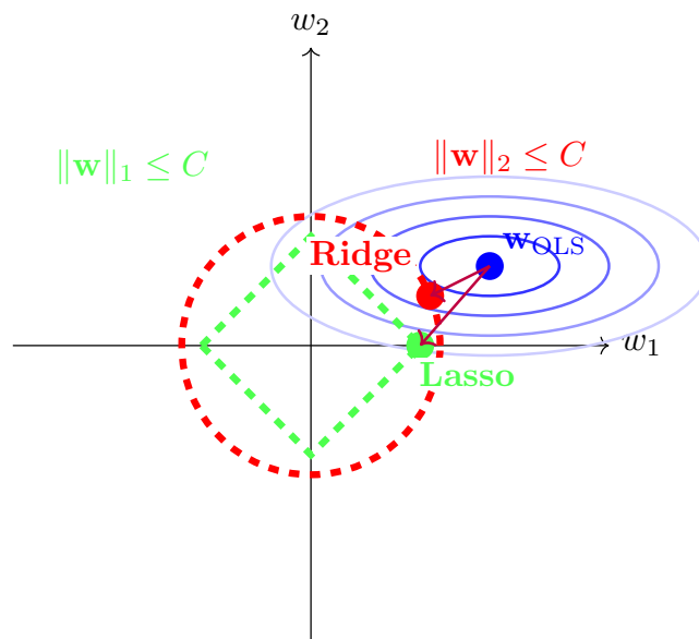
Figure 1.9.: Why the penalties behave differently: minimizing the loss subject to a weight budget. The spherical L_2 budget shrinks the solution toward the origin; the diamond-shaped L_1 budget has corners on the axes, so the solution tends to land where some coordinates are exactly zero (Exercise 5).
