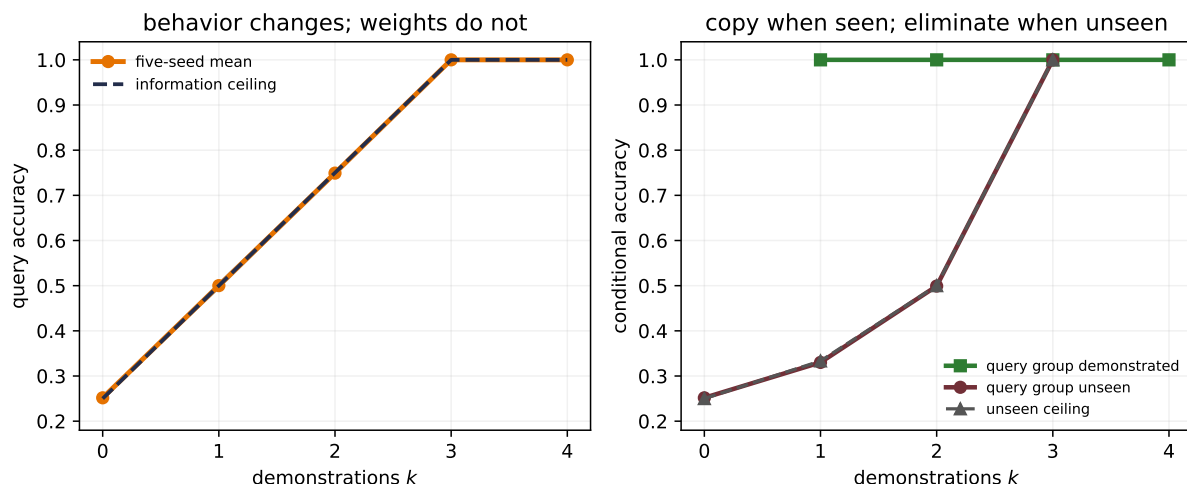
Figure 17.2.: A frozen model changes behavior as demonstrations reveal an episode’s hidden label mapping. Across five independently trained seeds, overall accuracy (left) tracks the exact information ceiling. Conditional accuracy (right) is perfect when the query group appeared; for unseen groups it follows the shrinking set of unused labels and reaches 1 at three demonstrations by elimination. Evaluation uses one nested episode bank per seed, and every parameter is bitwise unchanged across all five context lengths.
