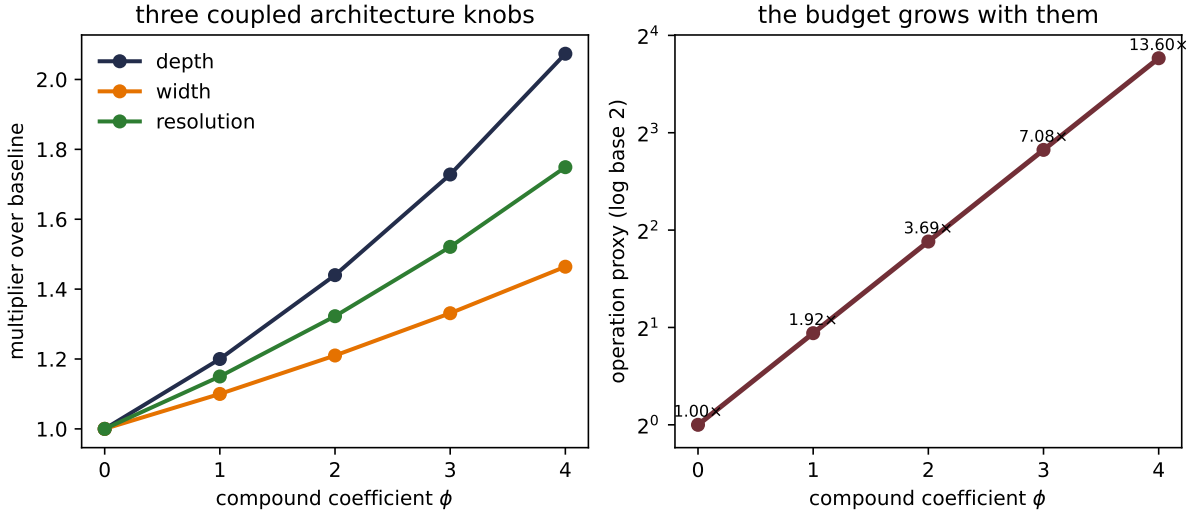
Figure 16.3.: EfficientNet’s published compound multipliers. Each step in \phi grows depth, width, and resolution modestly; their approximate convolutional-operation proxy grows by 1.92027 per step. These are normalized design multipliers, not measured accuracy or runtime.
