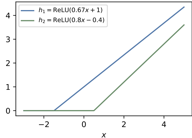
two hidden units
