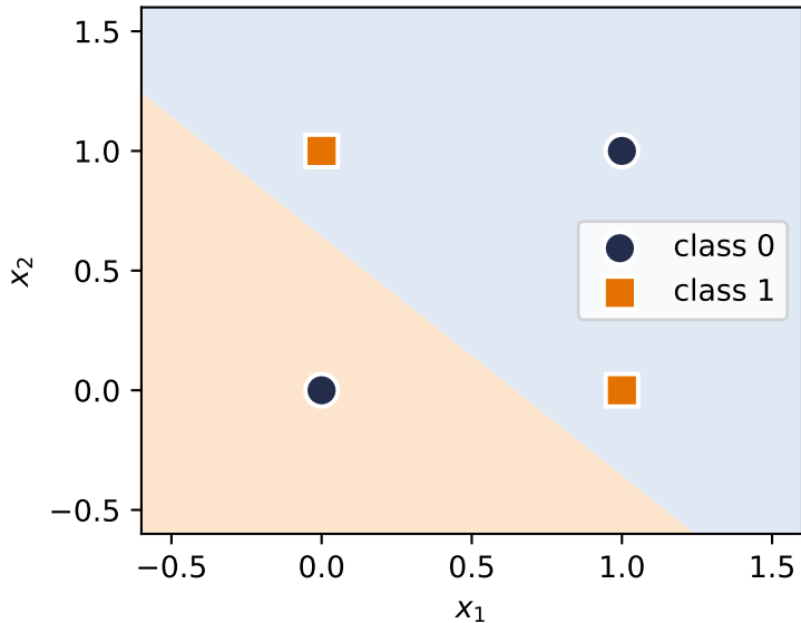
linear model
