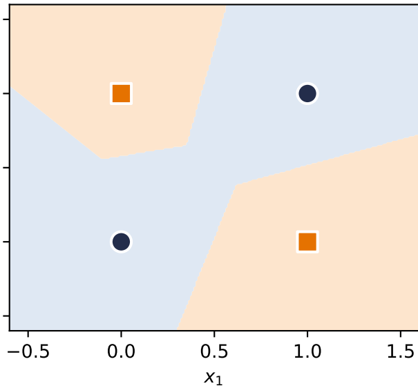
MLP with ReLU
