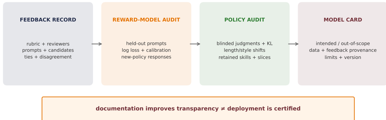
Figure 18.7.: Alignment evaluation is a chain of evidence, not one score. The feedback record identifies the rubric, reviewers, prompts, candidates, ties, and disagreement. Reward-model audits hold out prompts and test calibration and newer-policy responses. Policy audits add blinded judgments, realized KL, length and style shifts, retained capabilities, and relevant slices. A model card records intended and out-of-scope uses, data and feedback provenance, limitations, and versioning; it does not certify safety.
