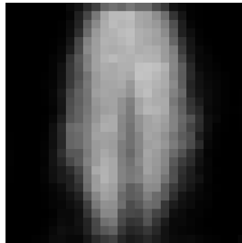
clean-trained AE
