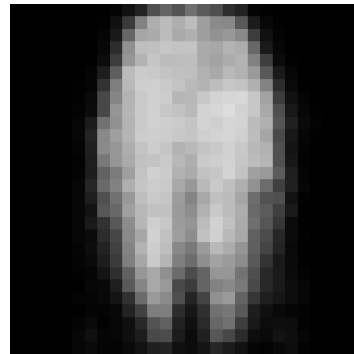
denoising AE
