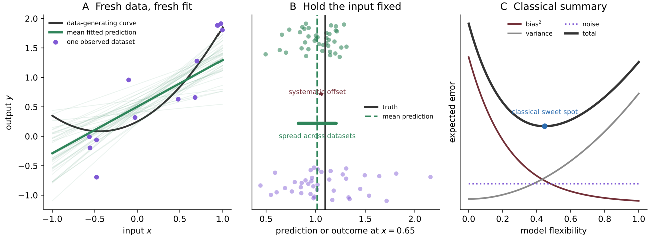
Figure 1.9.: Bias and variance, shown before they are named. Left: forty fresh noisy datasets produce forty fitted lines under one unchanged linear-regression recipe; one dataset is shown in purple, the mean fitted prediction in green, and the data-generating curve in black. Middle: at one fixed input, the prediction cloud has a systematic offset from the truth and a spread across training sets, while fresh outcomes retain their own noise. Right: the familiar U-curve compresses those three effects into a classical complexity cartoon. The seeded construction reveals the decomposition; it does not claim that every modern model follows one U-shaped path.
