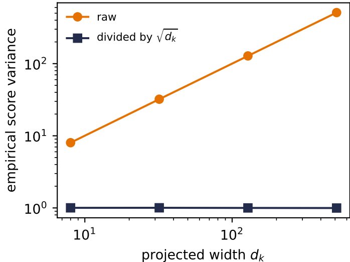
Control the score scale
