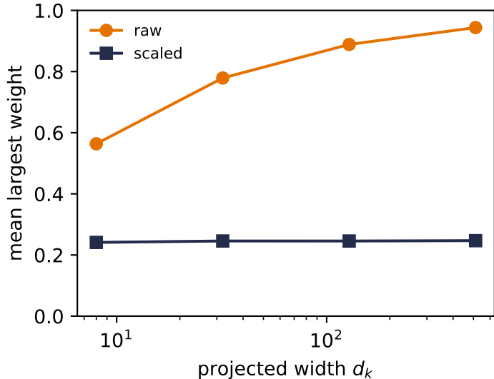
Control softmax concentration
