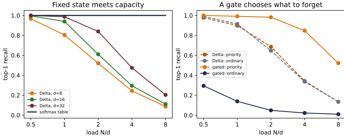
Figure 14.7.: A sealed synthetic mechanism test, not a language-model or state-space benchmark. Left: the uncompressed softmax table has perfect top-1 identification in this constructed, sharp-softmax regime, while the fixed delta state loses associations as N/d grows; this is not exact numeric interpolation. Right: the selective arm receives an unmatched priority bit and trades ordinary recall for priority recall. Keys, values, order, queries, decoder, and state width are matched within each trial; inference arithmetic, stored data, and side information are not matched, and no wall-clock claim is made. Left-panel lines average 30 endpoint seeds per dimension; right-panel lines pool the three dimensions, for 90 dimension-by-seed trials per load.
