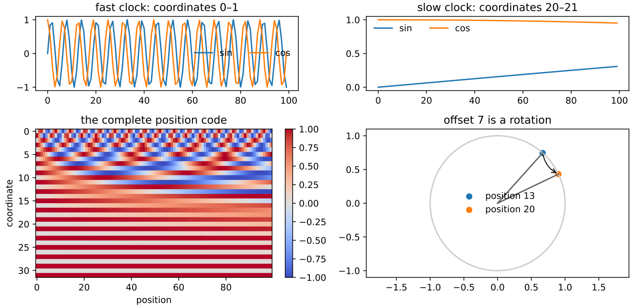
Figure 14.2.: Sinusoidal position is a bank of clocks. Fast coordinates track local offsets; slow coordinates vary across longer ranges. Each sine/cosine pair acts like a clock, and a fixed offset rotates that pair by a start-independent angle.
