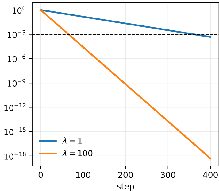
absolute eigencoordinate
