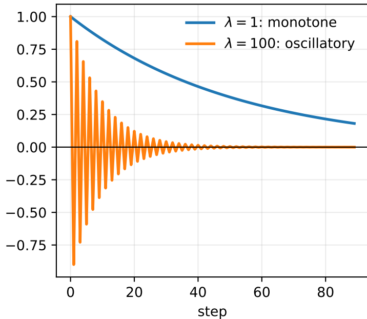
signed eigencoordinate
