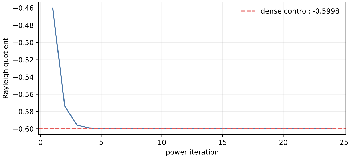
The dominant-magnitude curvature direction is negative
