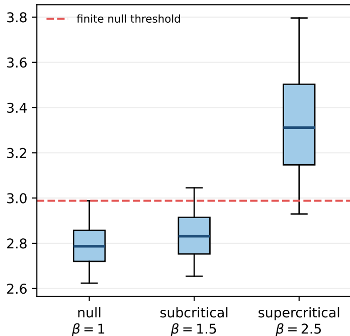
largest sample eigenvalue \lambda_{\max}
