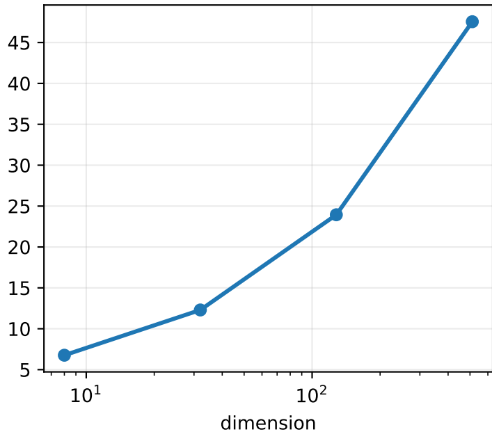
sub-Gaussian anchor threshold
