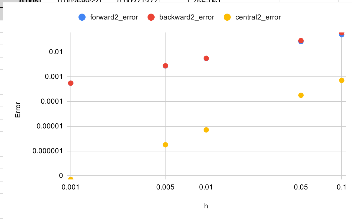
Figure-2: Error vs h (log-log) for second derivatives
