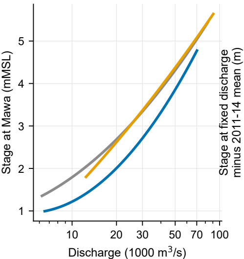
(a) Mawa rating curve by era
