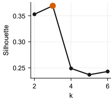
(b) Choice of k
