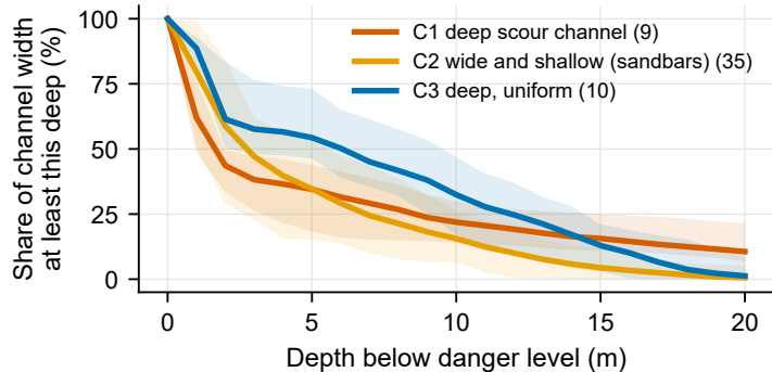
(a) Channel-shape clusters (hypsometry)
