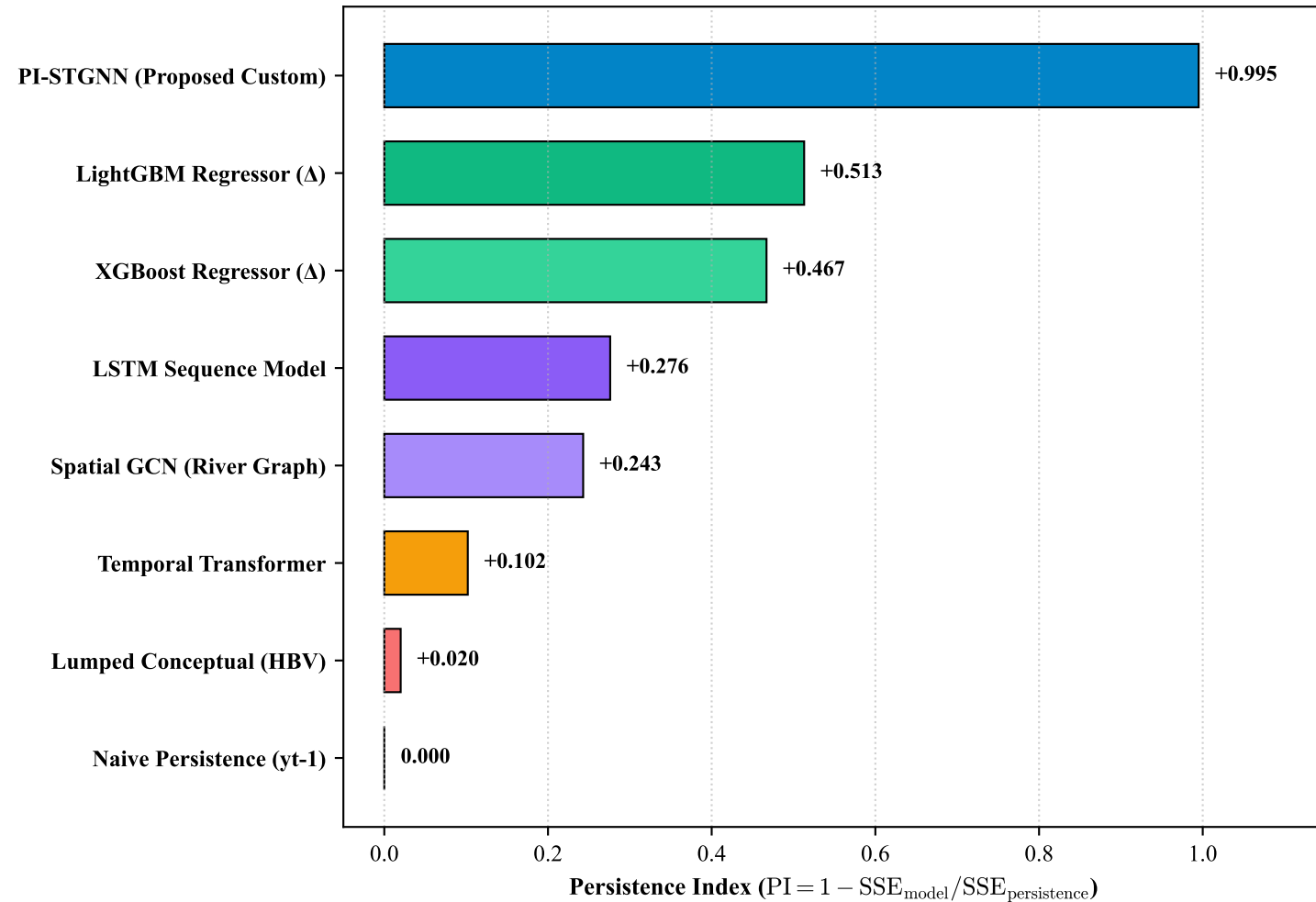
(a) Quantitative Benchmark: Persistence Gain over River Memory
