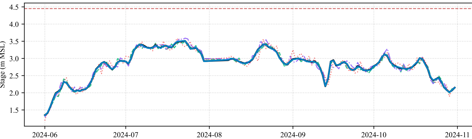
(e) 1-Day Ahead Forecast at Sureswar (Downstream Estuary) (SW95): 2024 Monsoon Season
