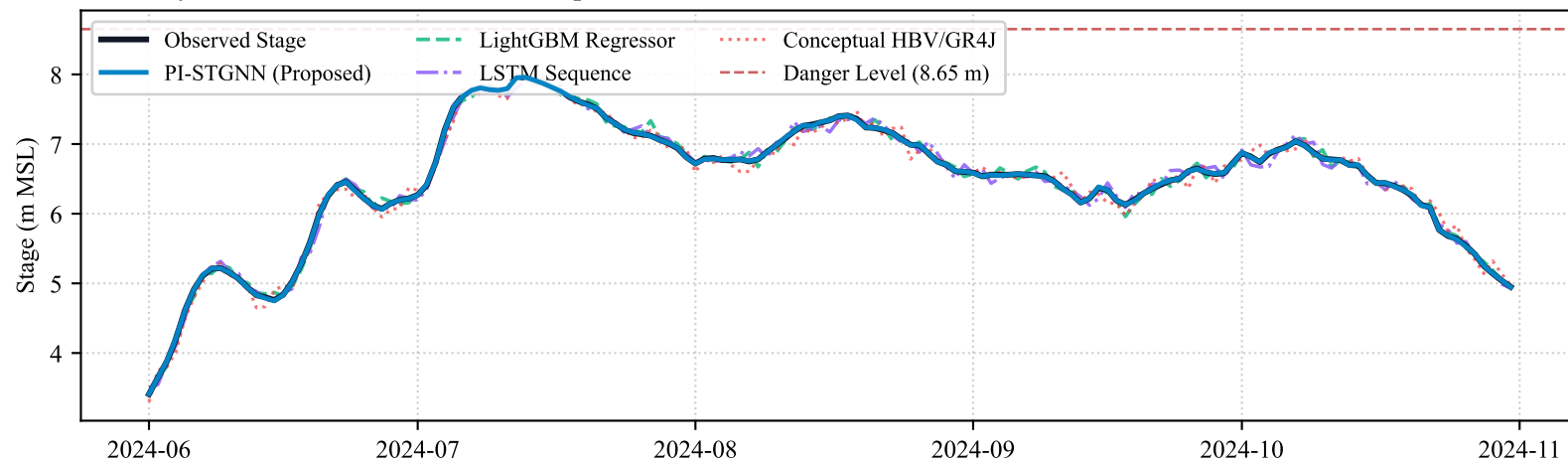
(a) 1-Day Ahead Forecast at Goalundo (Upstream Confluence) (SW91.9R): 2024 Monsoon Season
