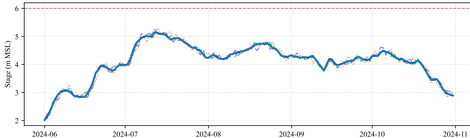
(c) 1-Day Ahead Forecast at Bhagyakul (Midstream Corridor) (SW93.4L): 2024 Monsoon Season
