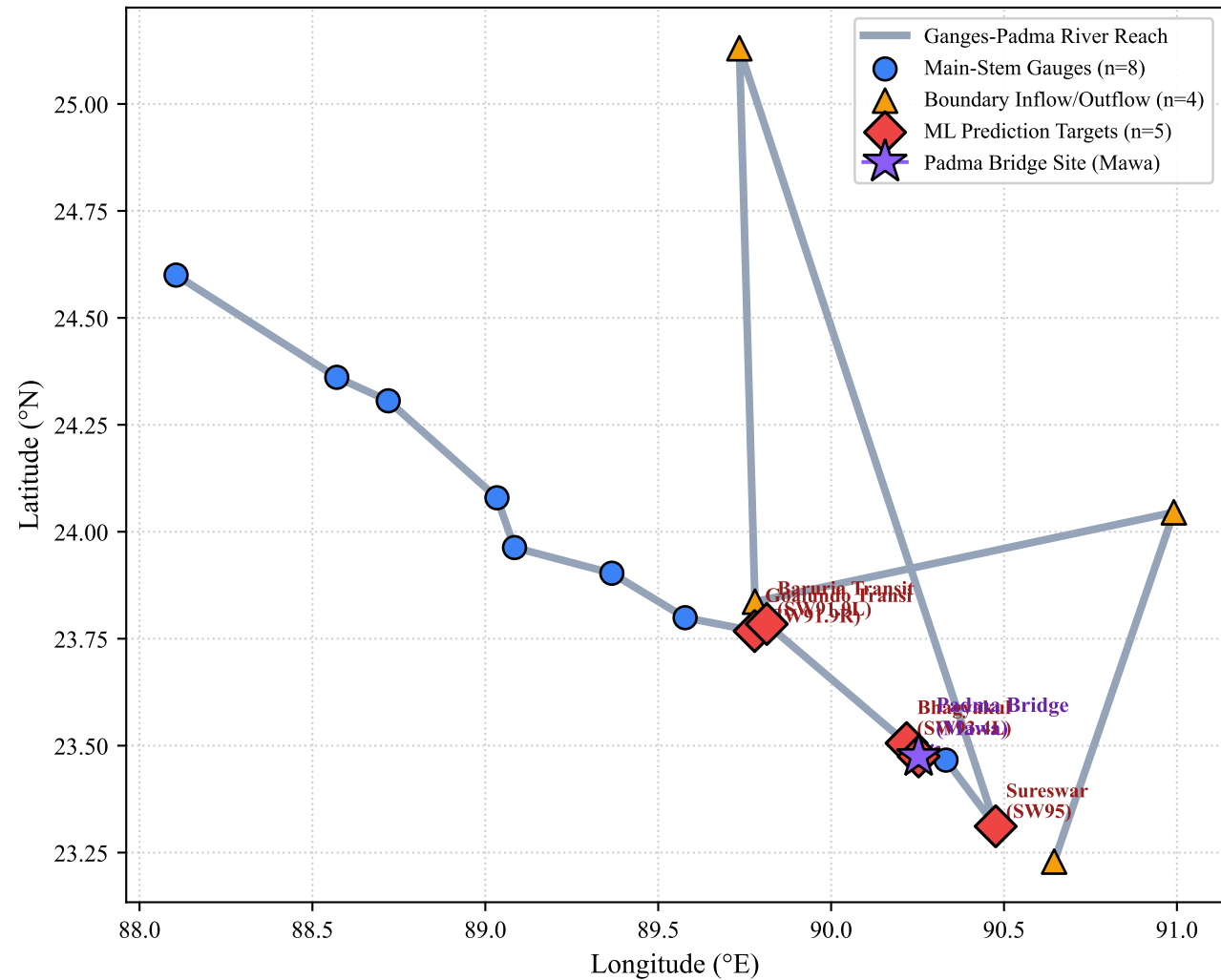
(a) Ganges–Padma Hydrometric Gauging Network
