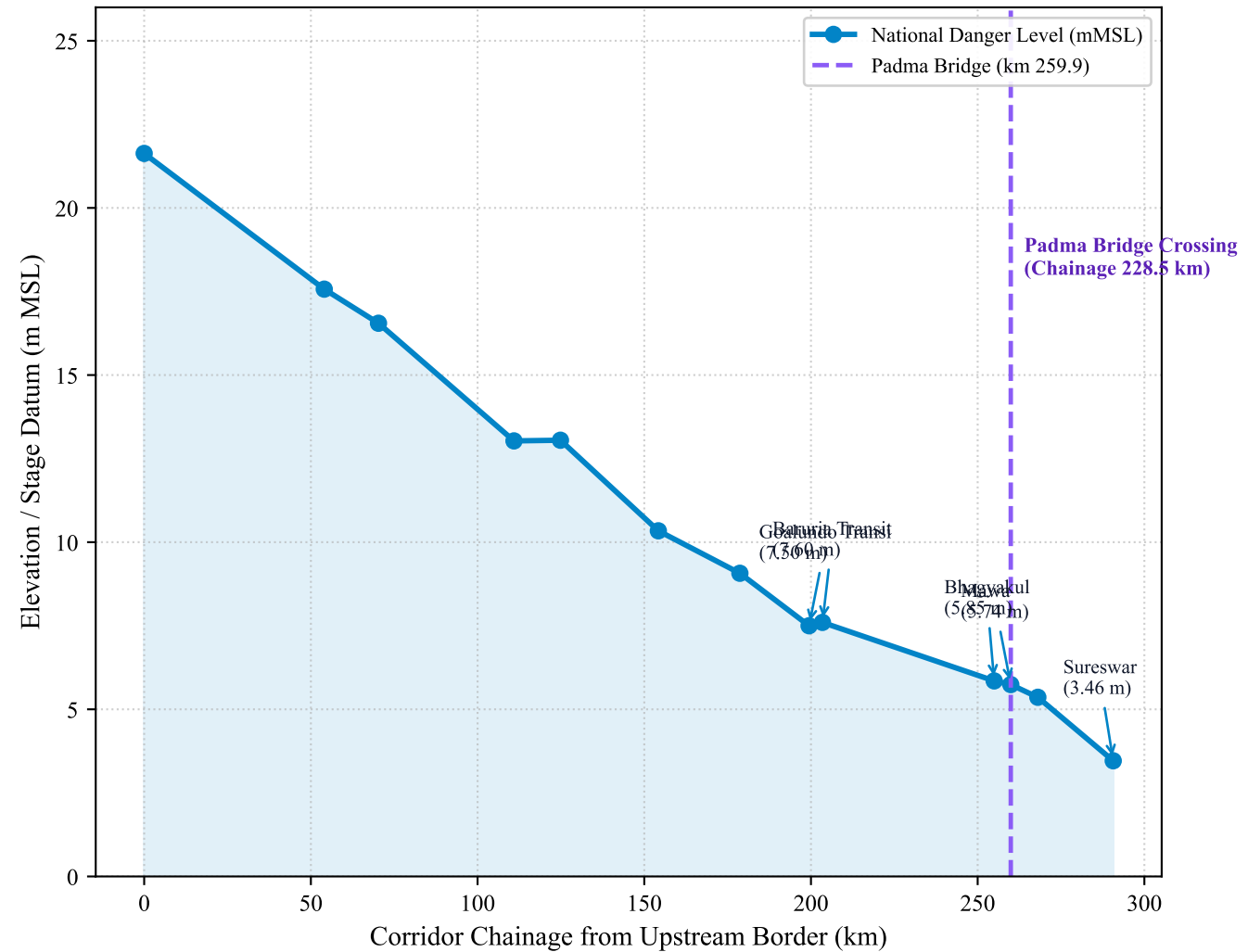
(b) Hydraulic Longitudinal Profile & Gauge Elevation Gradient
