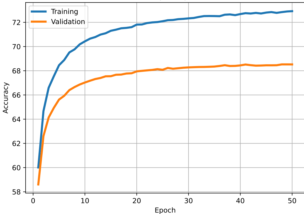
Accuracy vs Epoch
