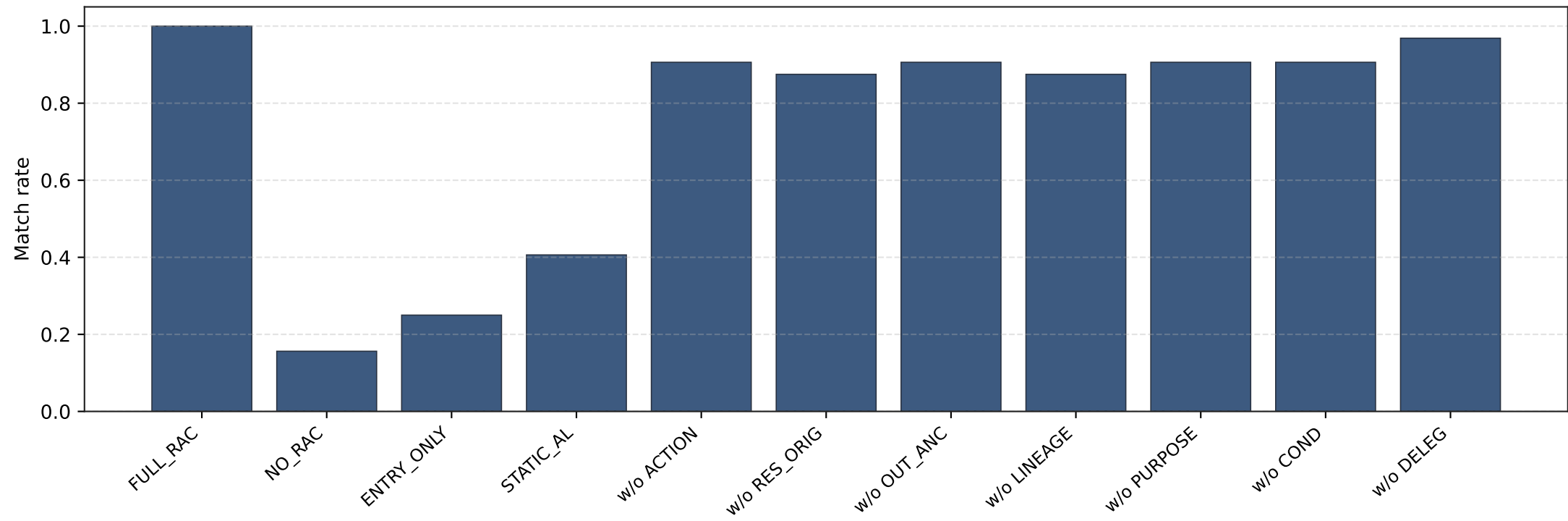
TraceBench v0.6: oracle match rate by replay variant (controlled replay)
