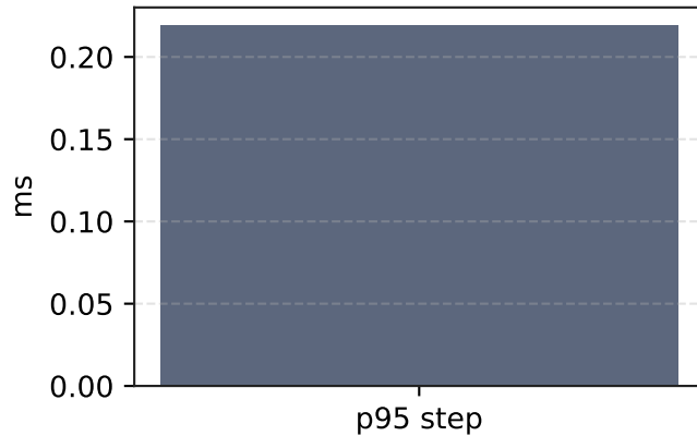
Overhead (microbenchmark)
