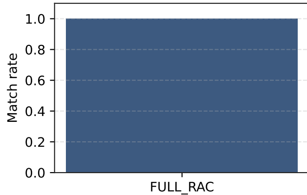
TraceBench (controlled)
