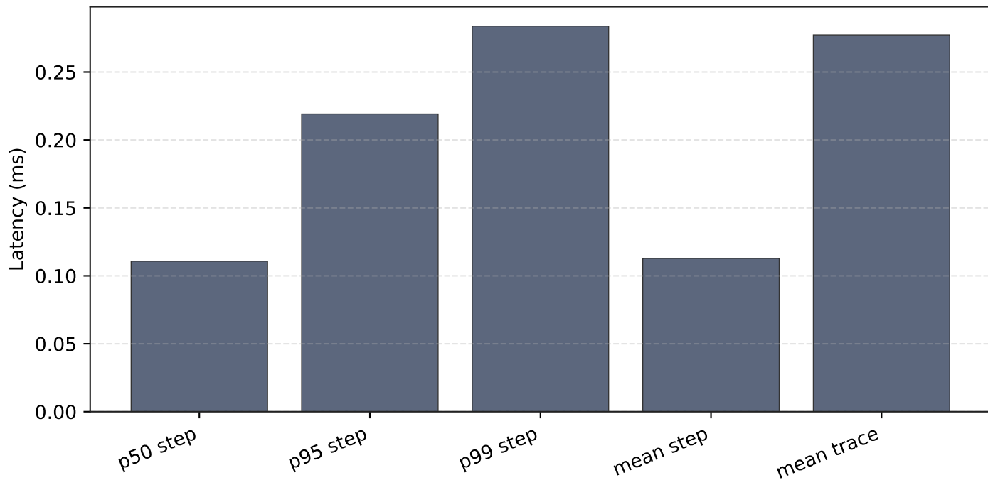
Controlled replay microbenchmark: step/trace latency (TraceBench harness)
