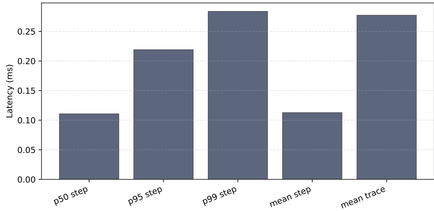
Controlled replay microbenchmark: step/trace latency (TraceBench harness)
