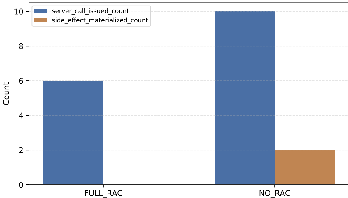
Planner filesystem MCP: issued calls vs write side-effects materialized
