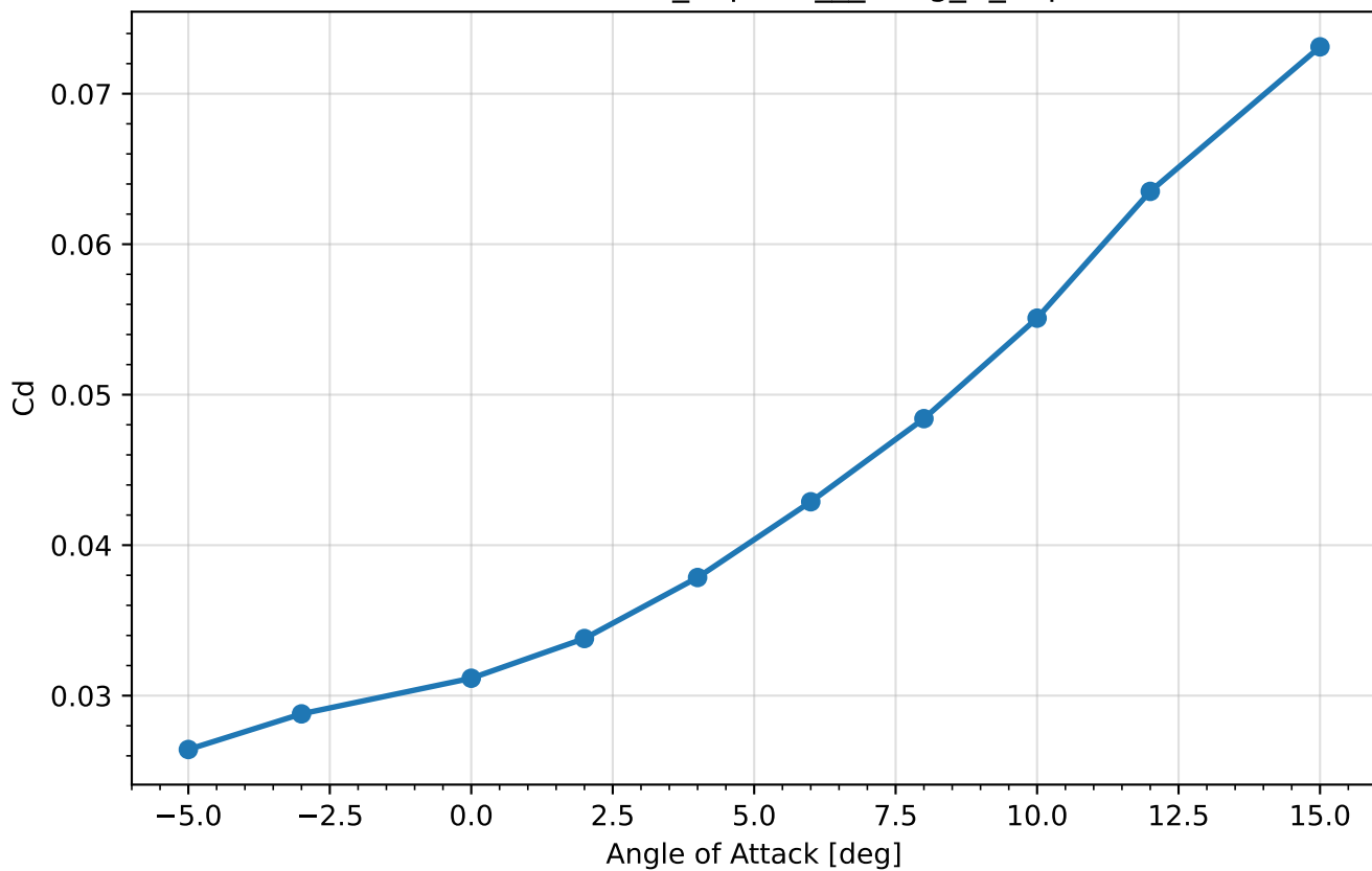
Cd vs AoA — cfd_exports__Wing_A_flap15
