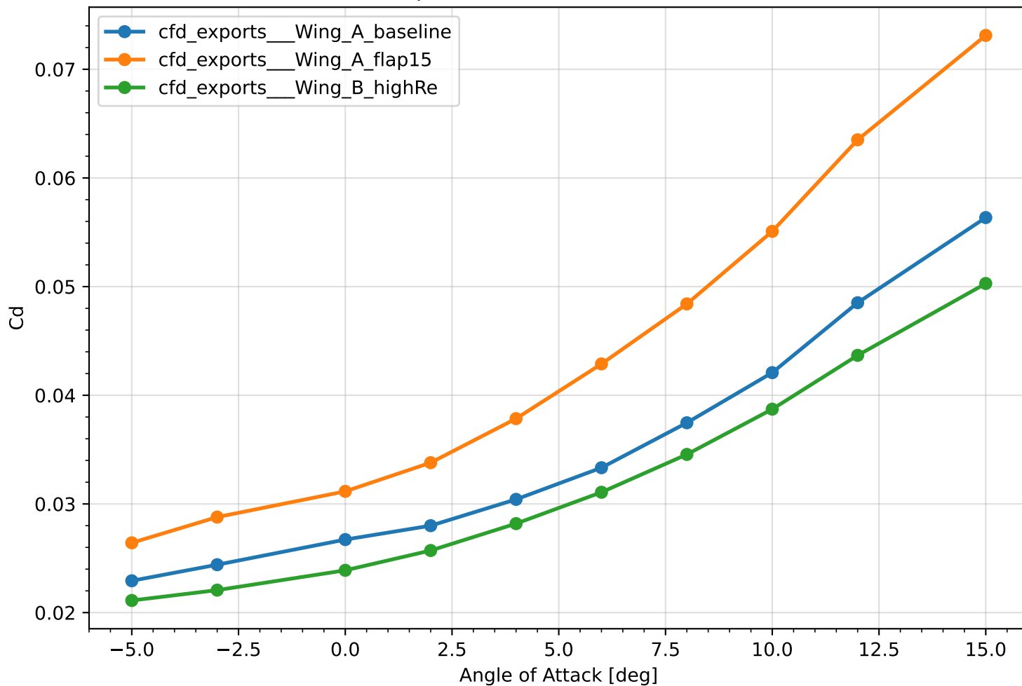
Comparison: Cd vs AoA (All Cases)
