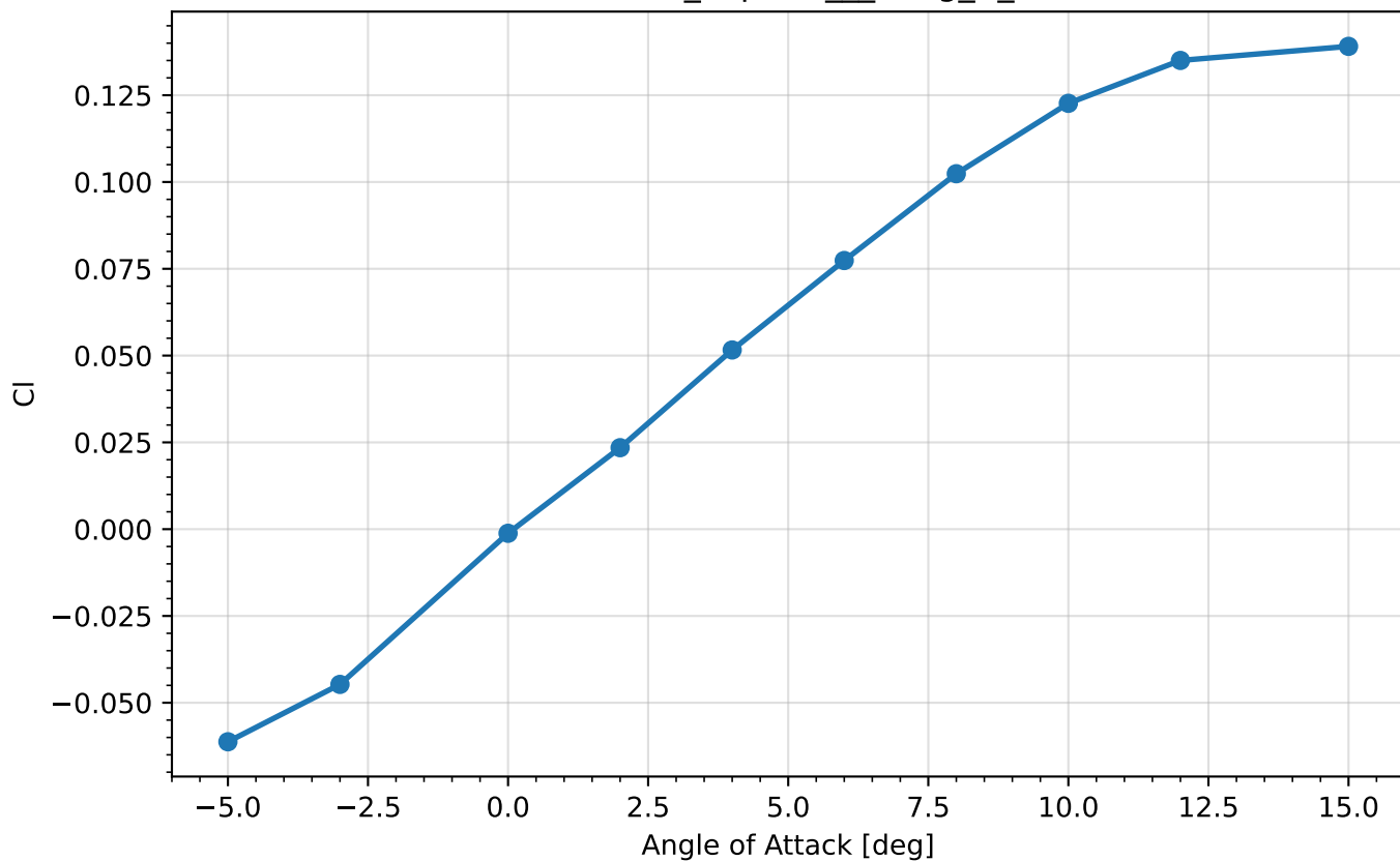
Cl vs AoA — cfd_exports__Wing_A_baseline
