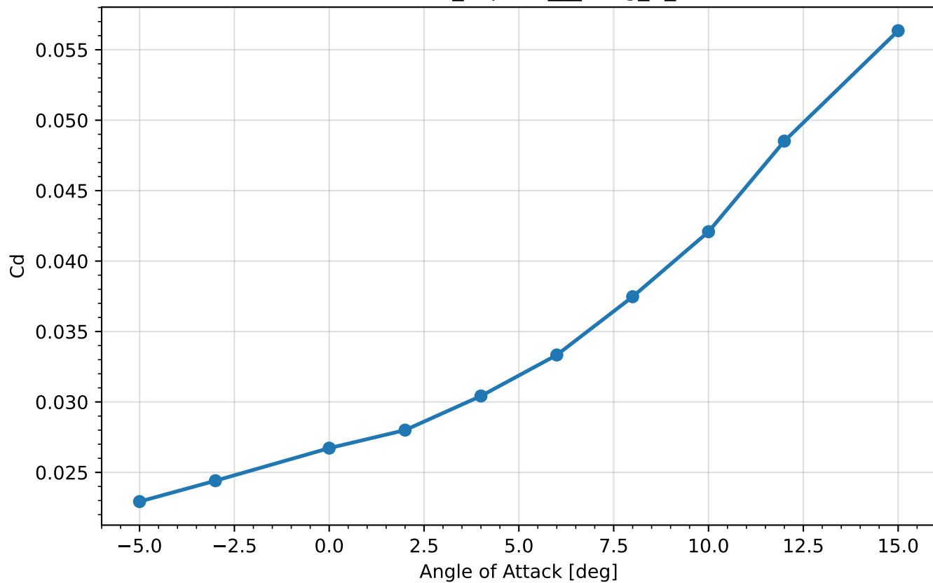
Cd vs AoA — cfd_exports__Wing_A_baseline
