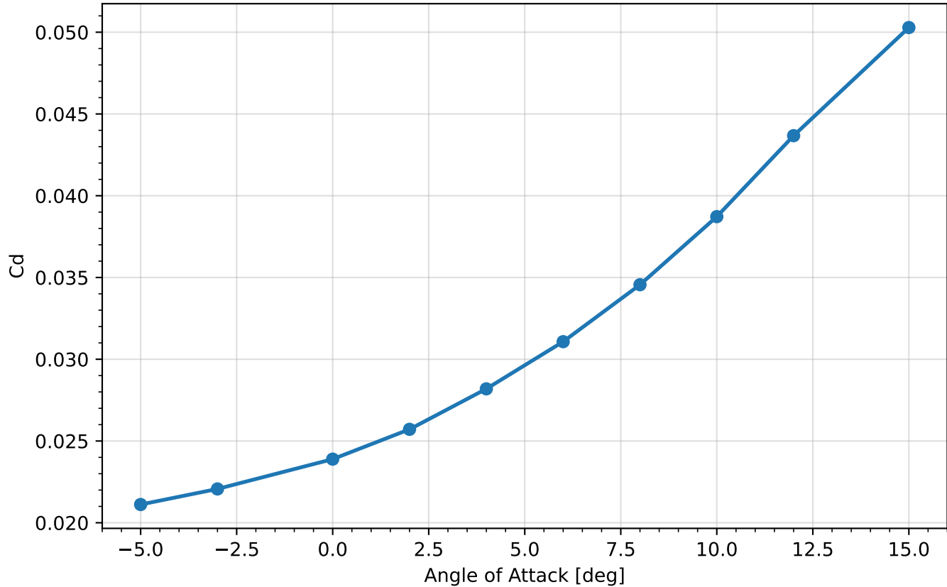
Cd vs AoA — cfd_exports__Wing_B_highRe
