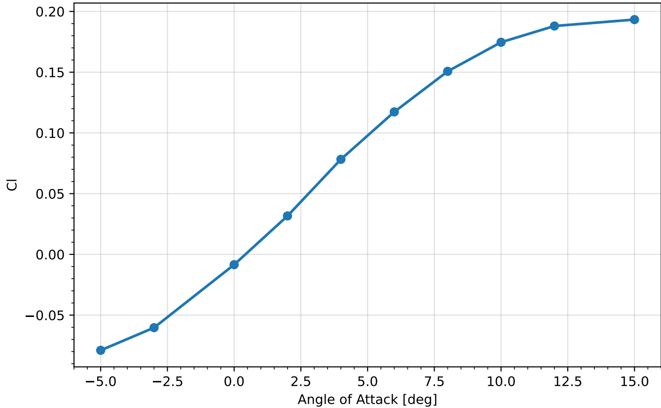
Cl vs AoA — cfd_exports__Wing_A_flap15
