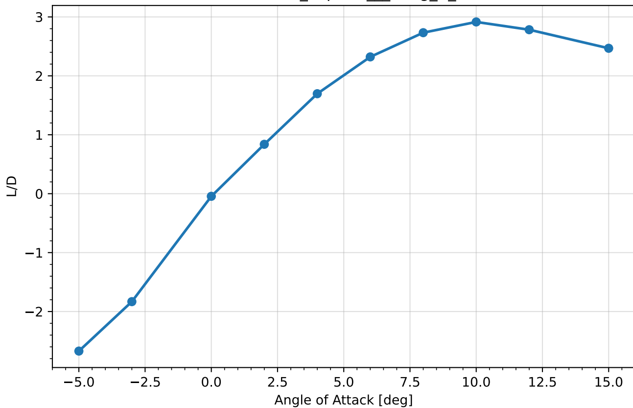
L/D vs AoA — cfd_exports__Wing_A_baseline
