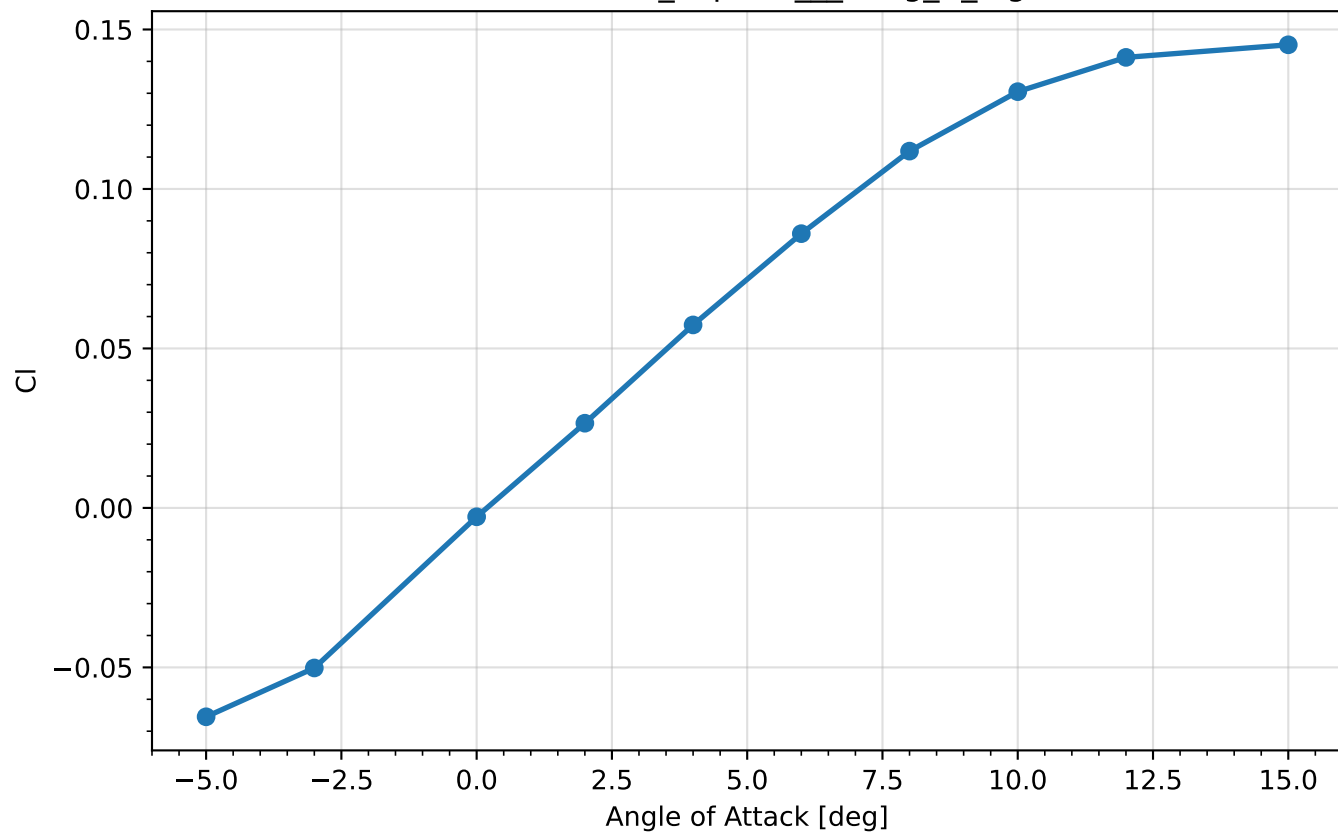
Cl vs AoA — cfd_exports__Wing_B_highRe
