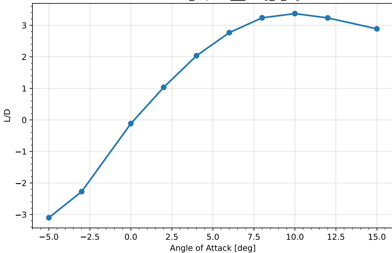
L/D vs AoA — cfd_exports__Wing_B_highRe
