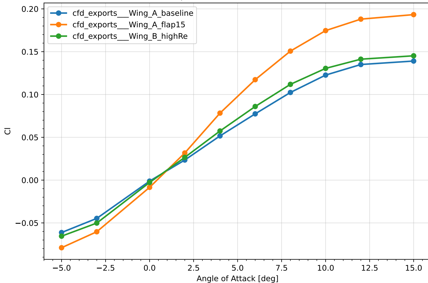
Comparison: Cl vs AoA (All Cases)
