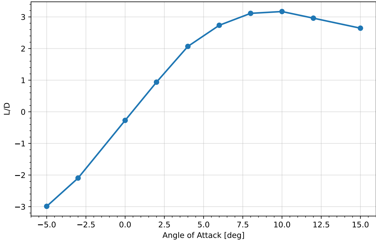
L/D vs AoA — cfd_exports__Wing_A_flap15
