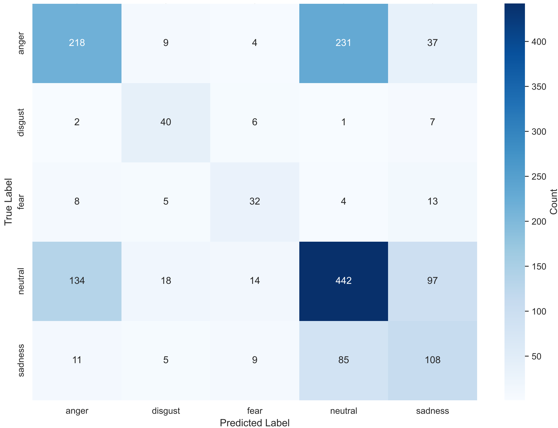
Confusion Matrix - Hybrid Fusion Model (Test Set, N=1540)
