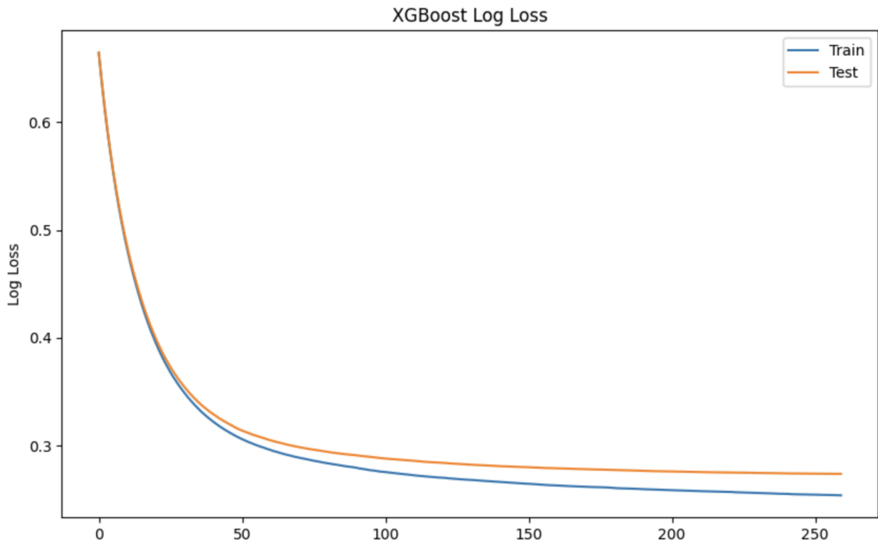
Plot 1: Logloss Plot over 260 epochs ( n\_estimators = 260 )
