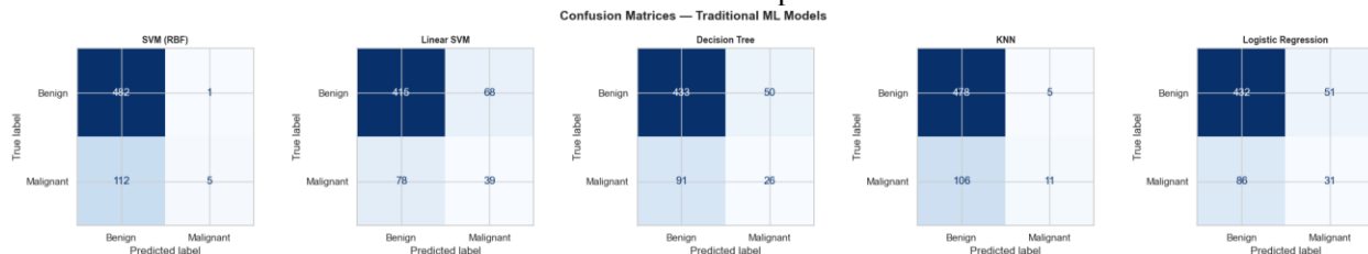
Figure 13.1: Traditional ML Baseline Confusion Matrices (SVM-RBF, Linear SVM, Decision Tree, KNN, Logistic Regression)
