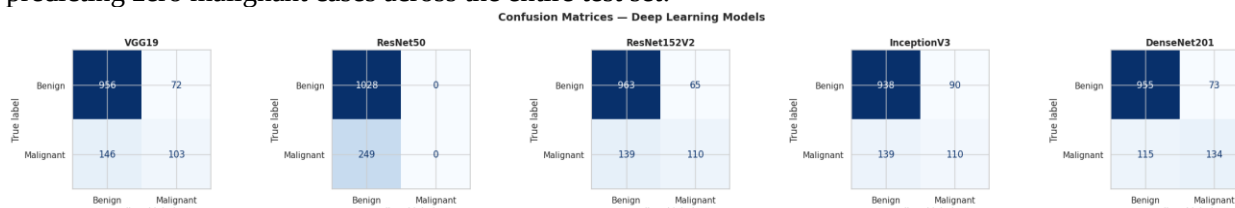
Figure 14.1: Deep Learning Baseline Confusion Matrices (VGG19, ResNet50, ResNet152V2, InceptionV3, DenseNet201)
