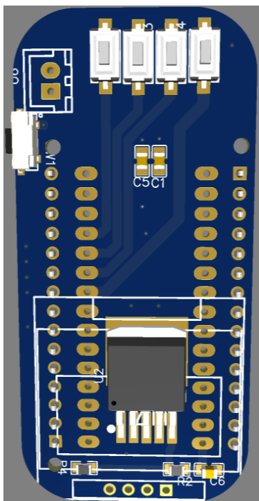
Figure 37: 3D top view of the wearable gesture recognition device PCB.
