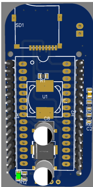
Figure 38: 3D bottom view of the wearable gesture recognition device PCB.
