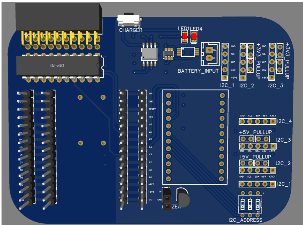
Figure 41: 3D view of the top side of the learning platform PCB.
