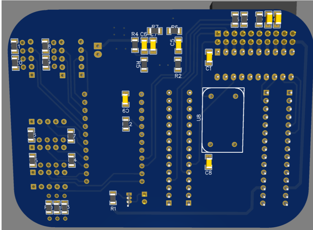
Figure 40: 3D view of the bottom side of the learning platform PCB.
