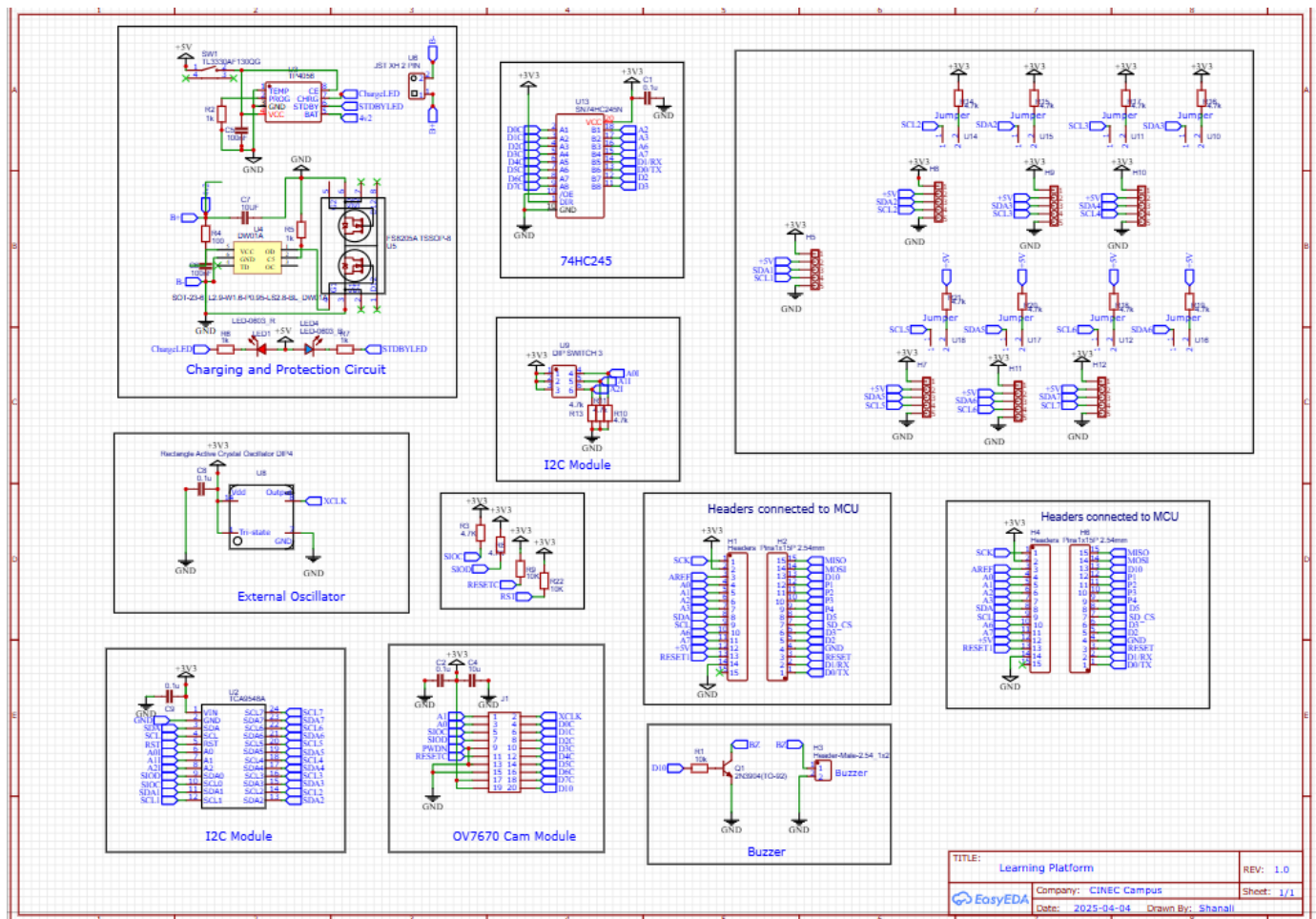
Figure 39: Schematic design of the learning platform.
