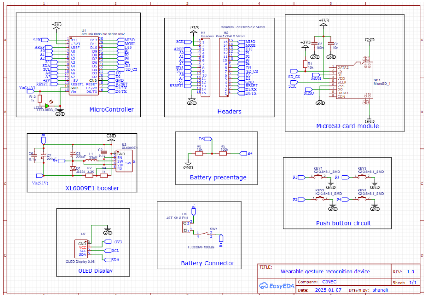
Figure 36: Schematic design of the wearable gesture recognition device.
