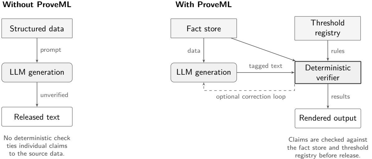
Figure 3: Without ProveML (left): data goes in, text comes out, no verification. With ProveML (right): every claim is checked against the fact store and threshold registry, with an optional correction loop. Rounded boxes denote generative components; squared boxes denote data stores and deterministic processing.
