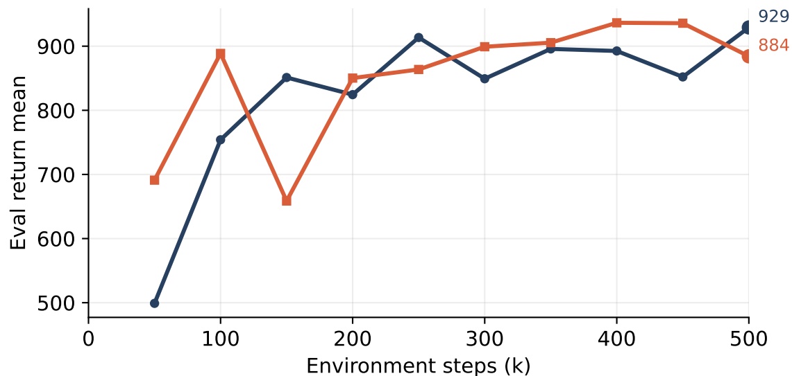
cheetah-run / clean
