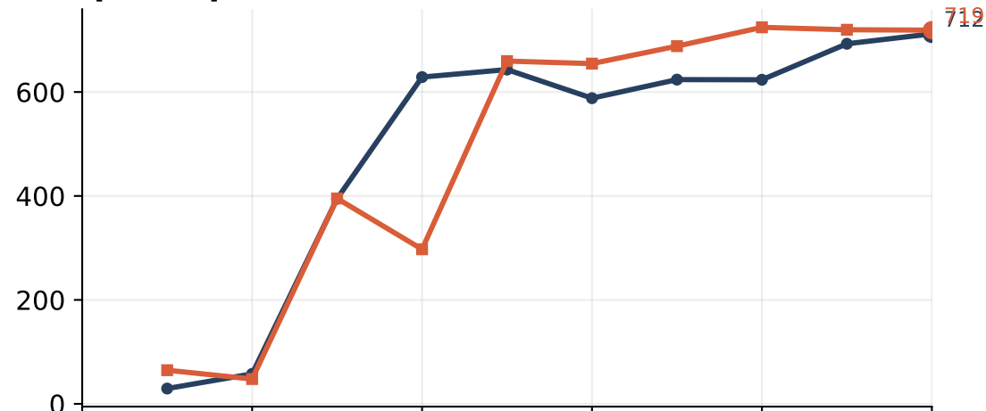
quadruped-run / chaos
