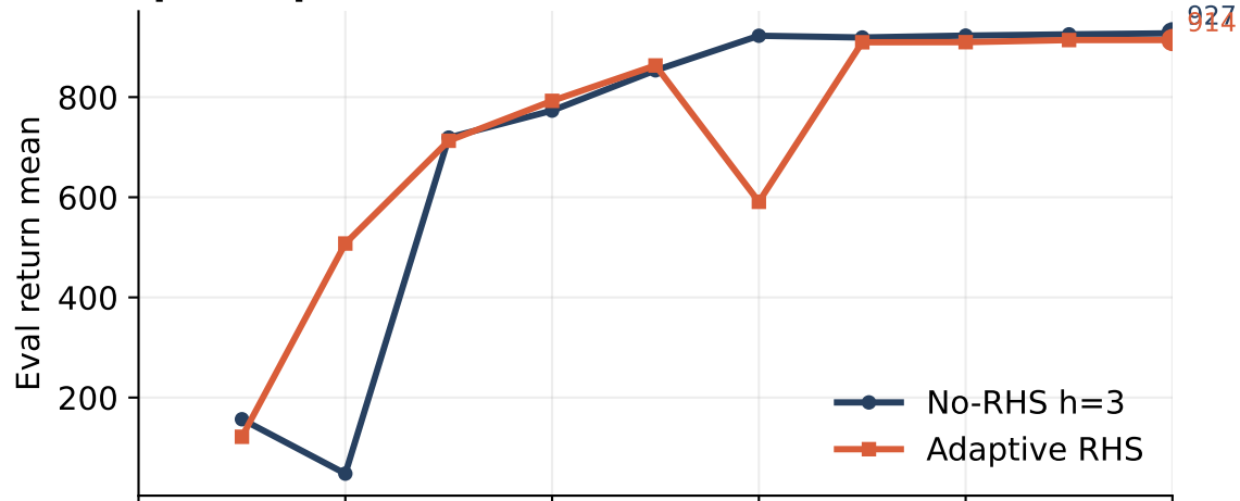
quadruped-run / clean
