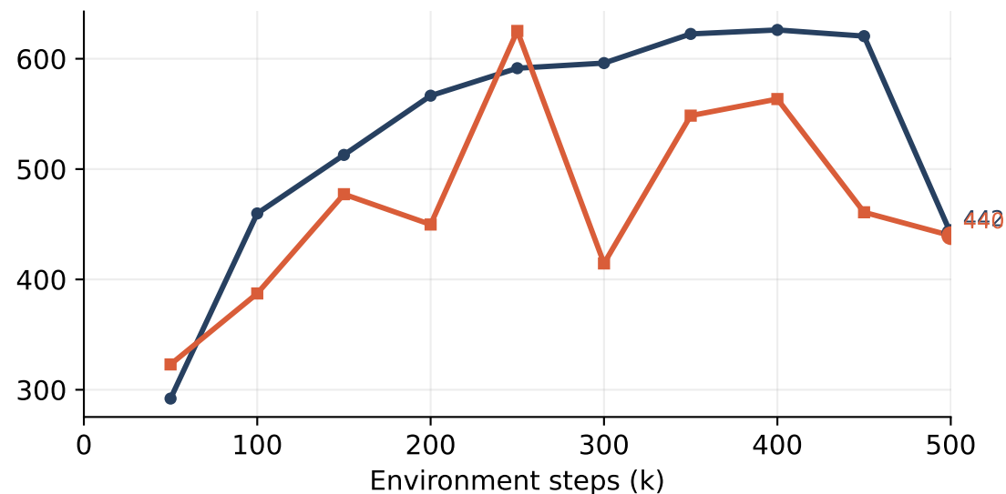
cheetah-run / chaos
