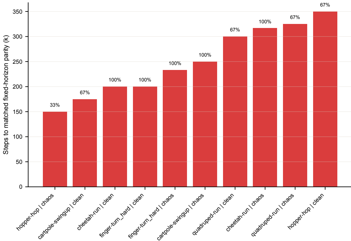
Sample efficiency: reaching matched baseline final score
