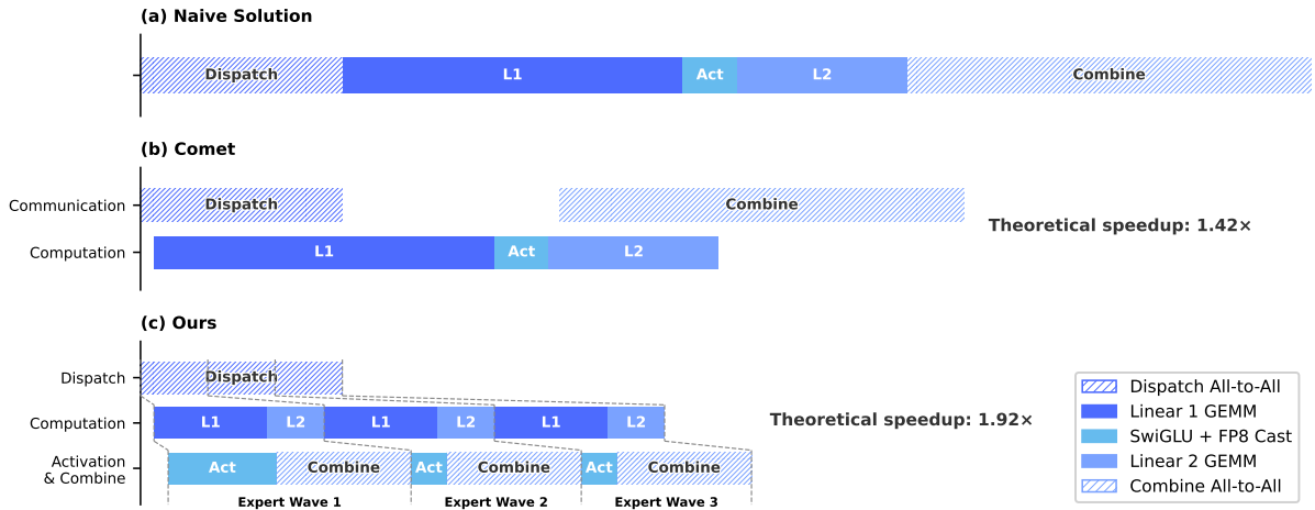
Figure 5 | Illustration of our EP scheme with related works. Comet ( Zhang et al., 2025b ) overlaps Dispatch with Linear-1, and Linear-2 with Combine, separately. Our EP scheme achieves a finer-grained overlapping by splitting and scheduling experts into waves. The theoretical speedup is evaluated in the configuration of the DeepSeek-V4-Flash architecture.
