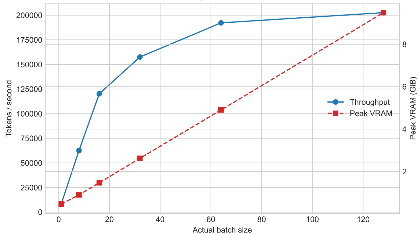
Batch scaling on RTX 4080 SUPER
