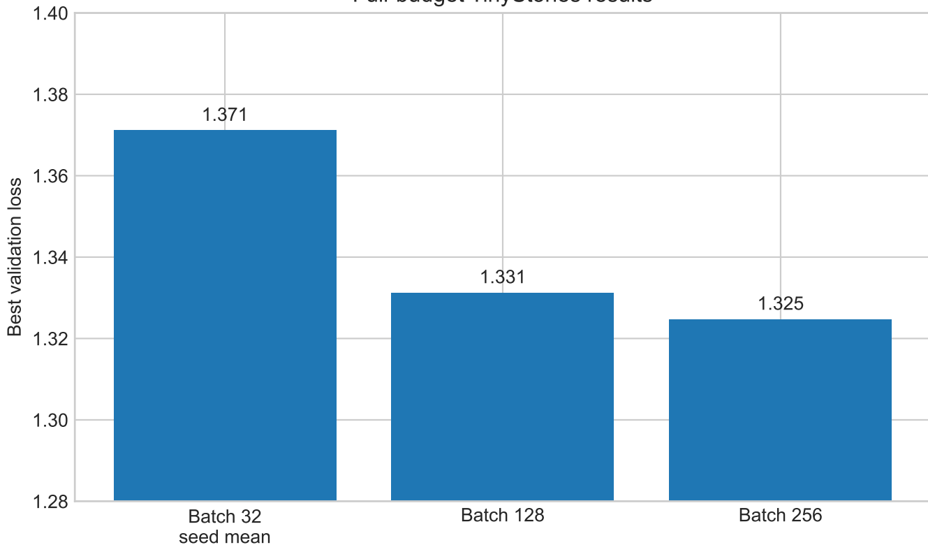
Full-budget TinyStories results
