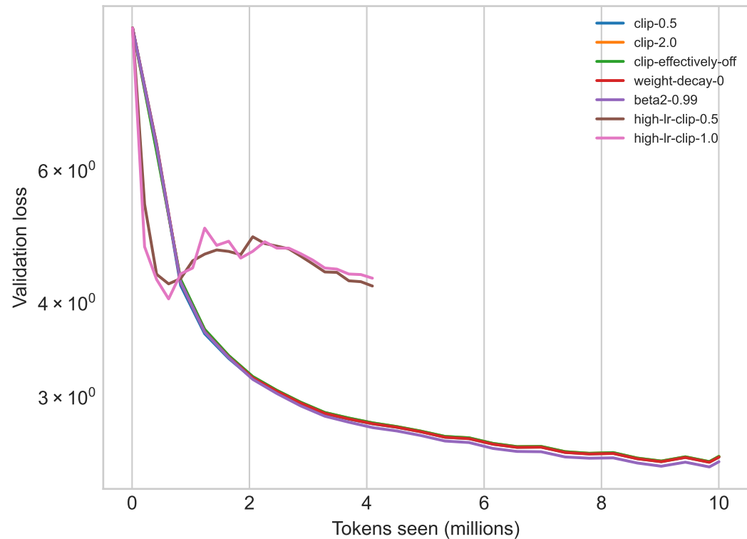
Optimizer generalization
