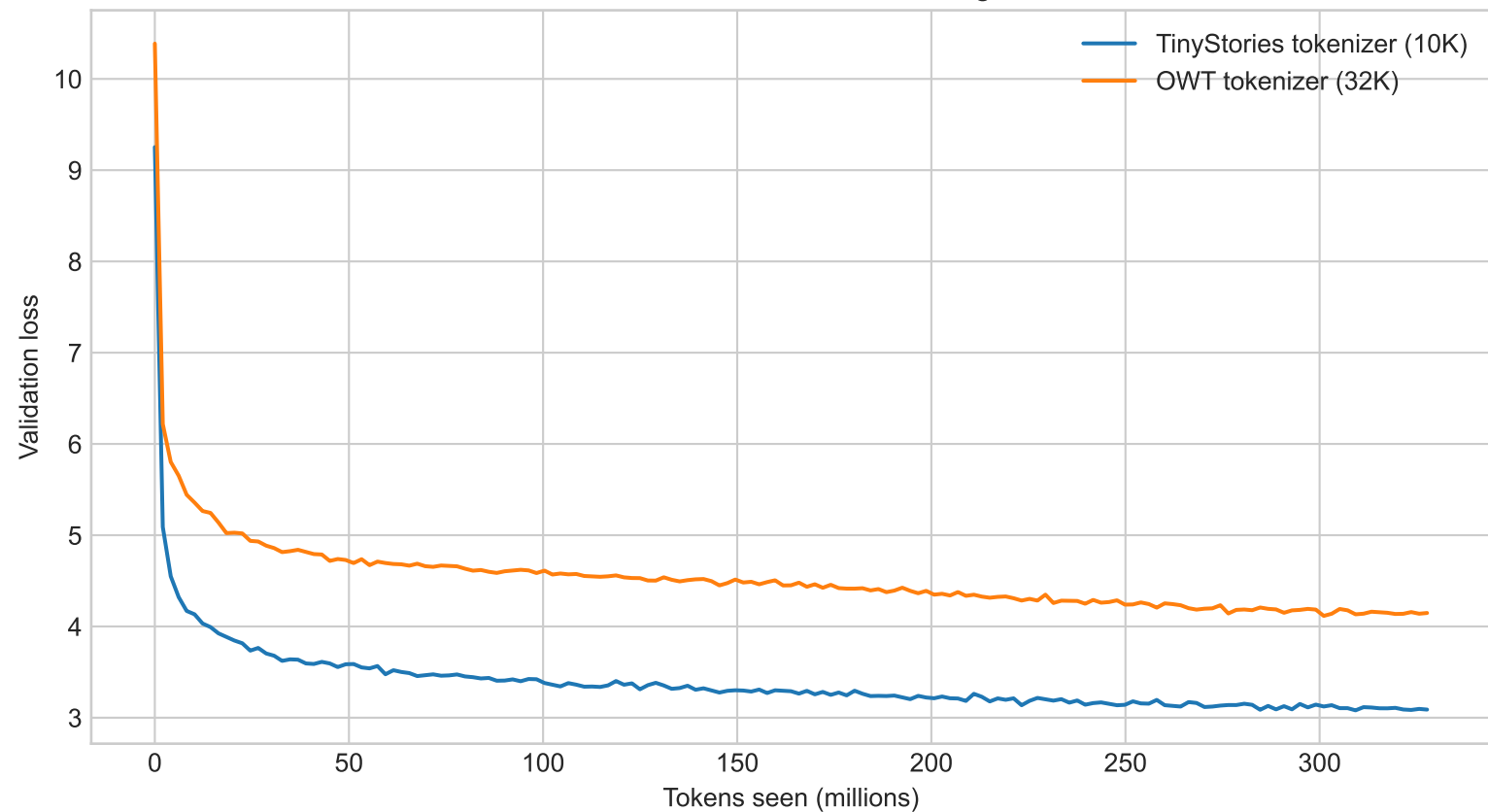
OWT cross-tokenizer training
