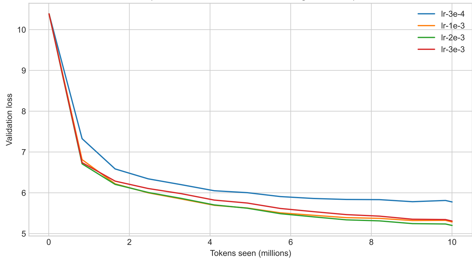
OpenWebText 32K-tokenizer learning-rate sweep
