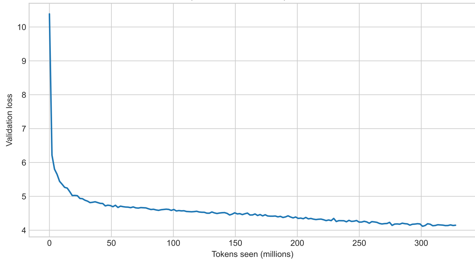
OpenWebText main experiment
