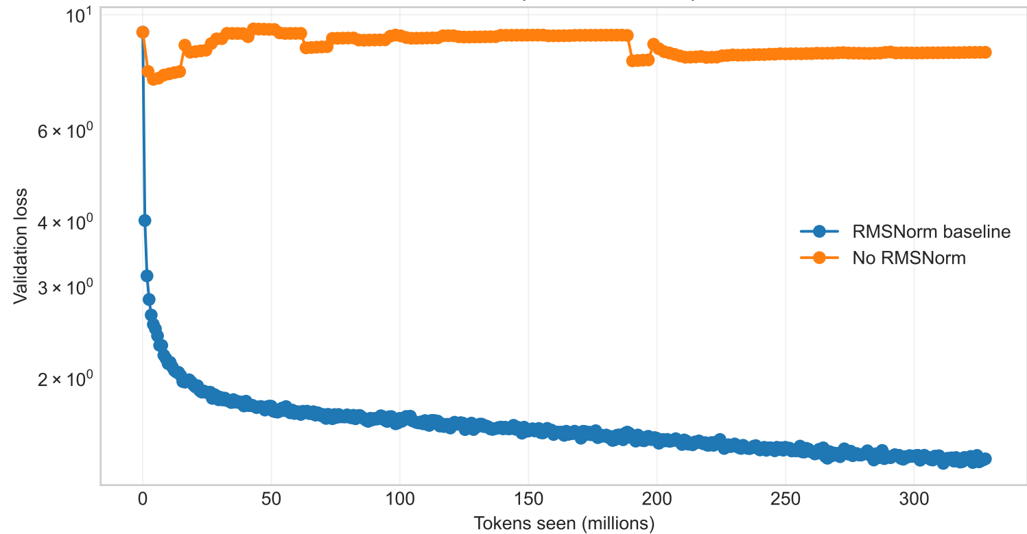
Normalization is required for stable optimization
