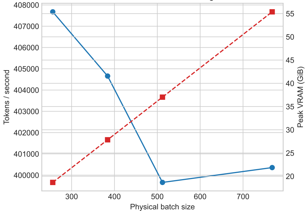
RTX 6000D batch scaling
