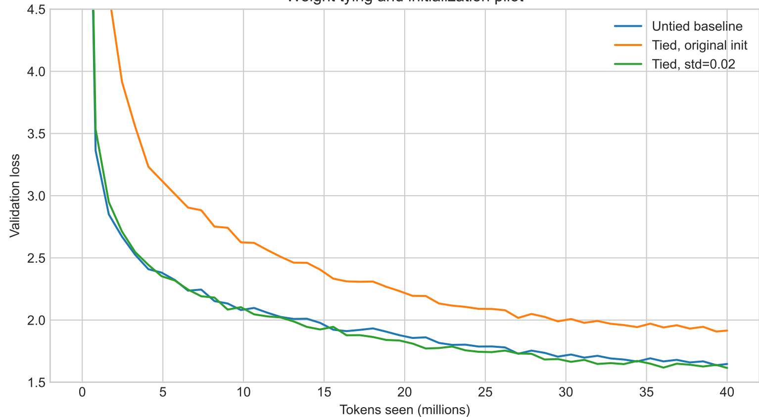
Weight tying and initialization pilot
