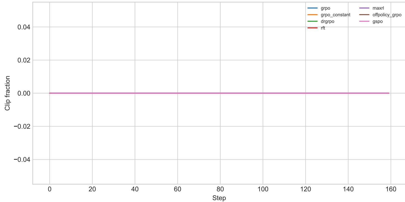
Off-policy clipping
