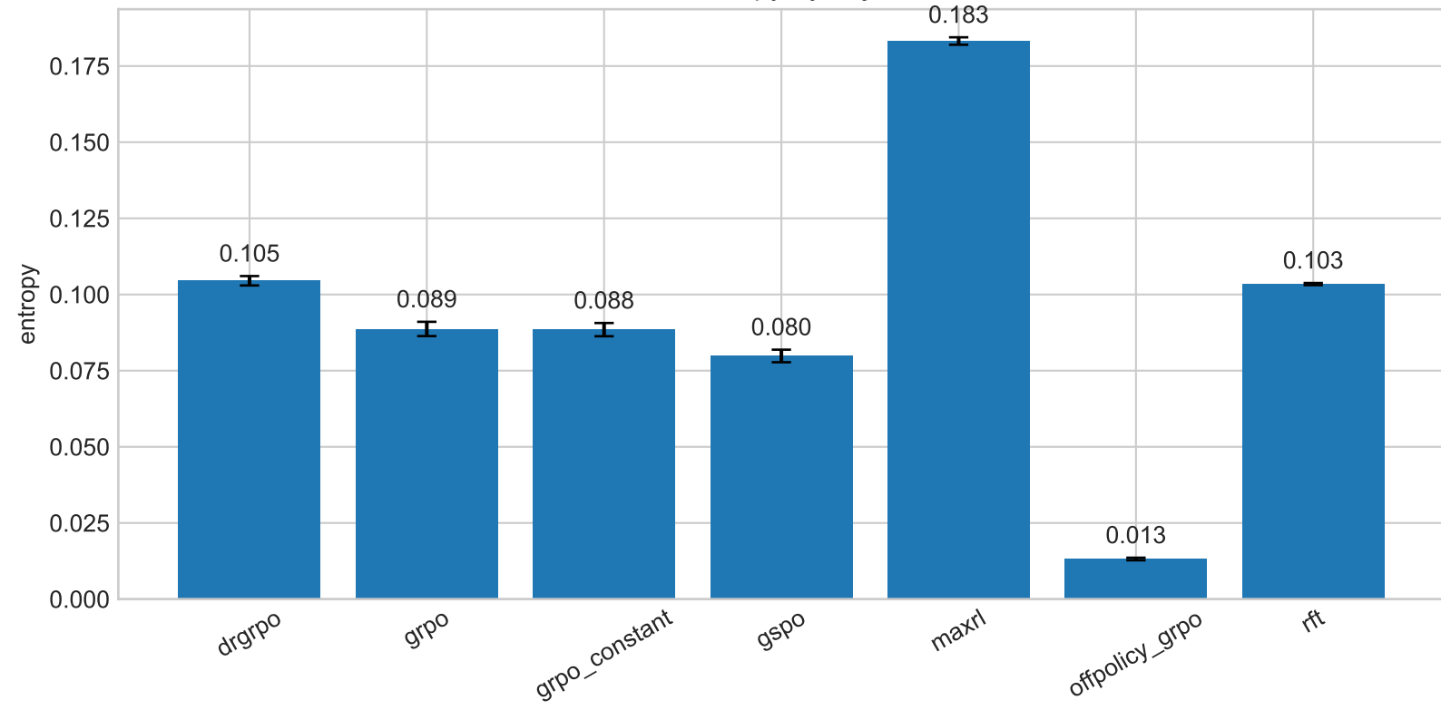
Final entropy by objective
