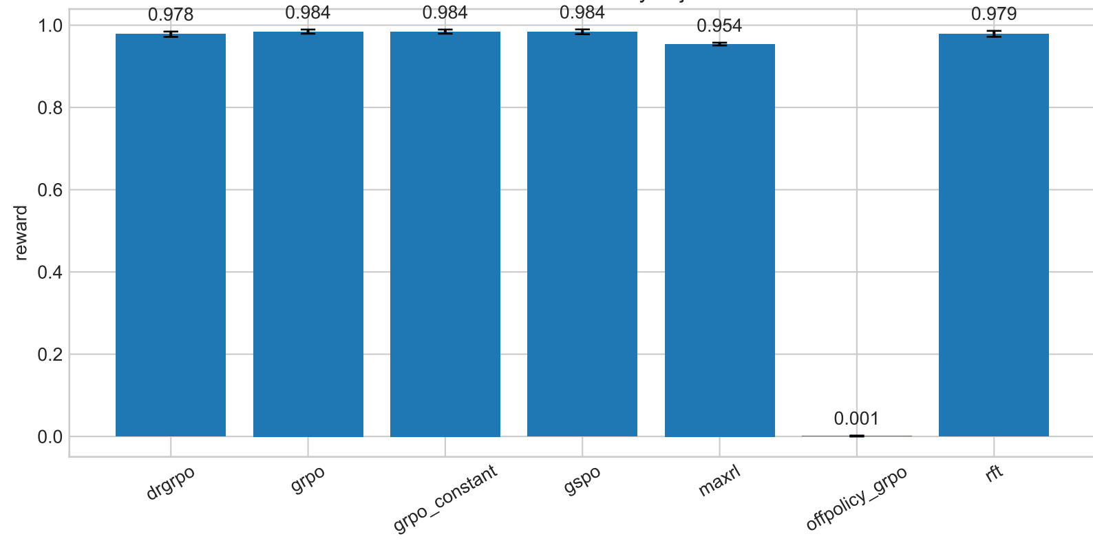
Final answer reward by objective
