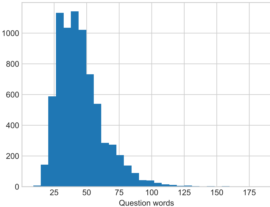
GSM8K question length
