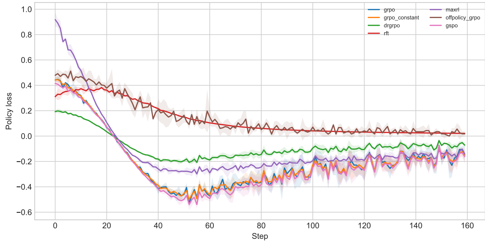
Surrogate optimization
